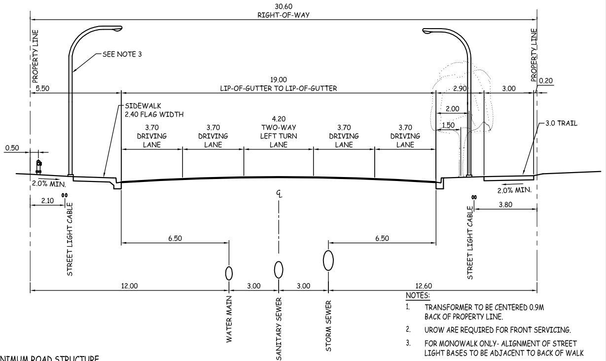
WITH TWO-WAY LEFT TURN LANE
